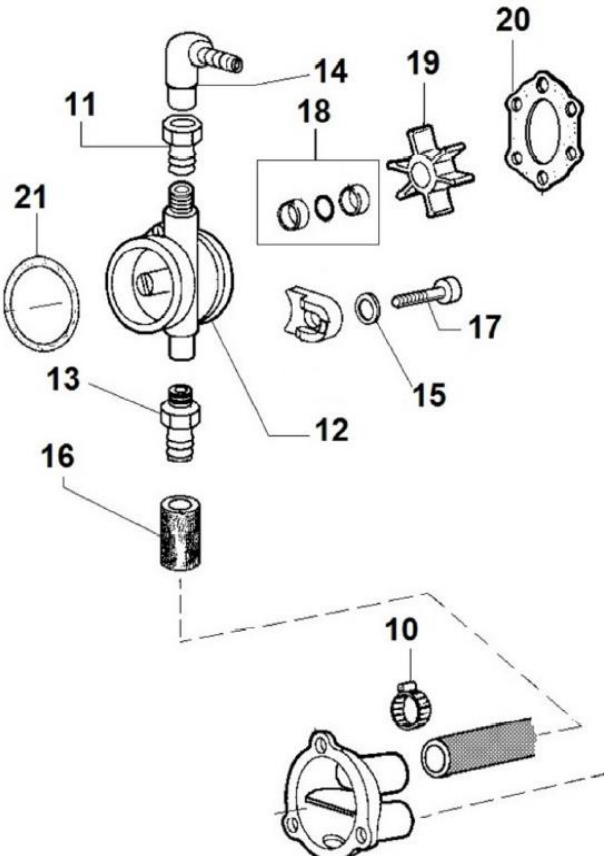
PAGURO - SPARE PARTS CATALOGUE PAGURO 6000 - COOLANT PUMP
